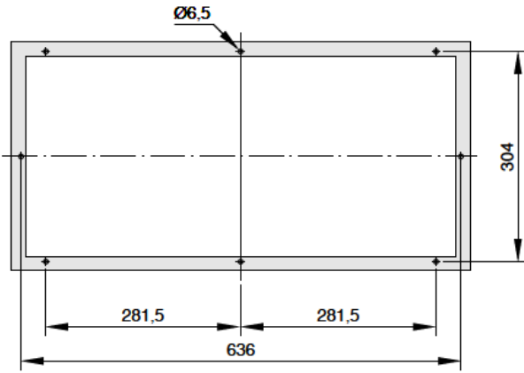
TFW flange dimensions
